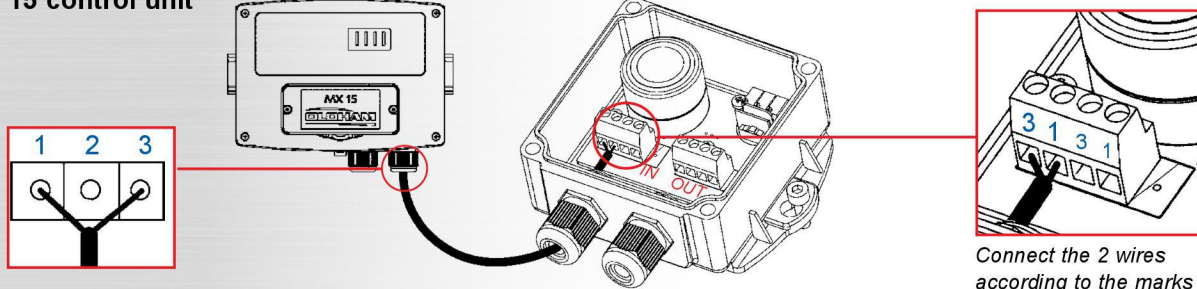
MX 15 control unit
